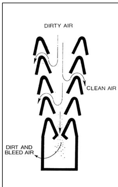
Figure 4: Dynavane Dust Separation (9)
