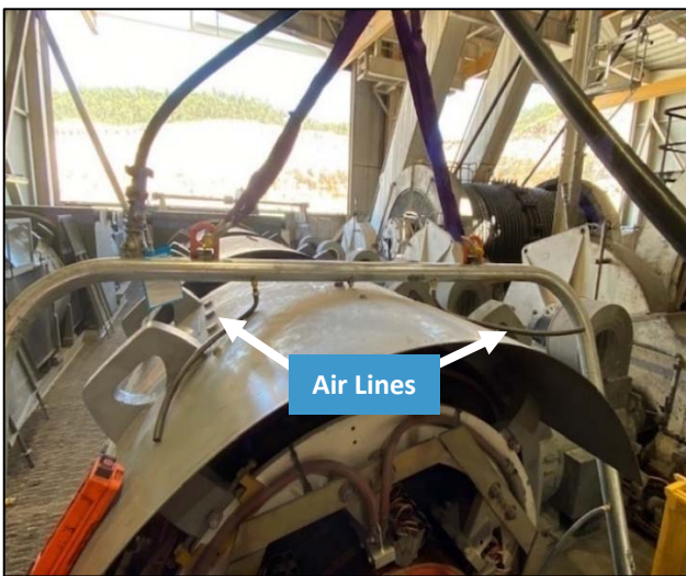
Photos 23 & 24: remotely operated dust agitator with compressed air line for MG sets suspended from overhead crane
