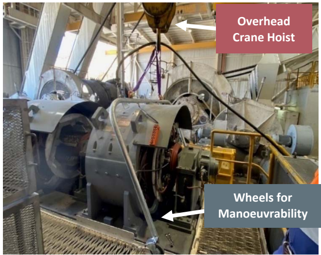
Photos 23 & 24: remotely operated dust agitator with compressed air line for MG sets suspended from overhead crane
