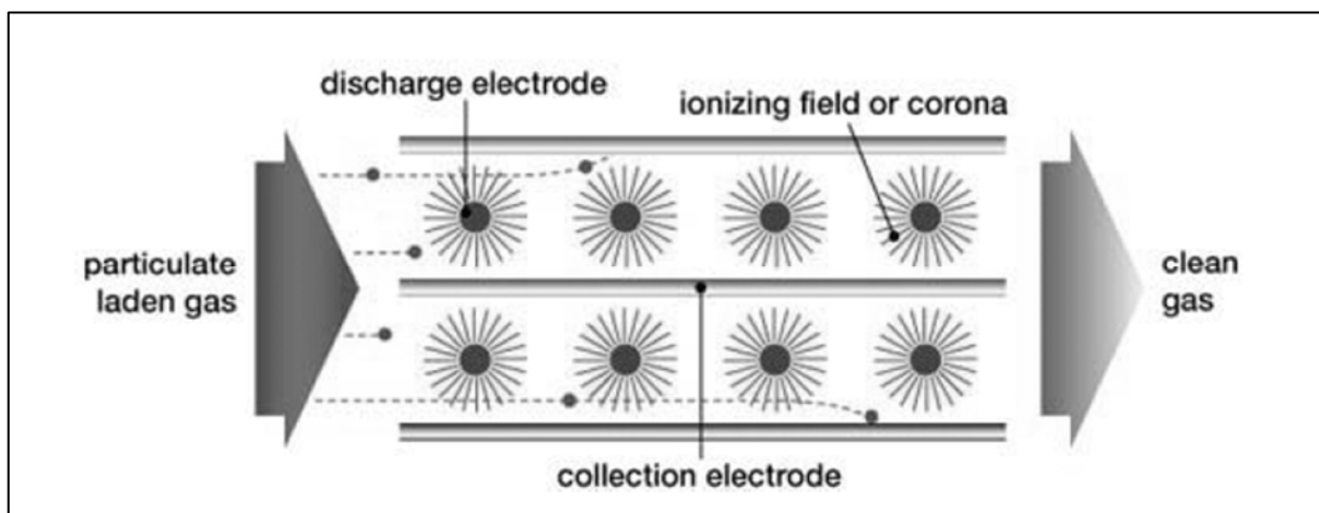
Figure 8: Example of electrostatic dust precipitation (10)
