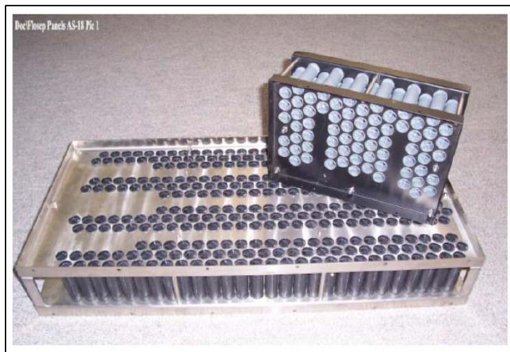
Photo 13: Flosep panels comprising multiple individual tubes (picture supplied by Flosep Dust Filtration Australia) (9)
