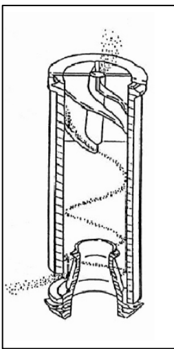
Figure 7: Individual Flosep device (9)
