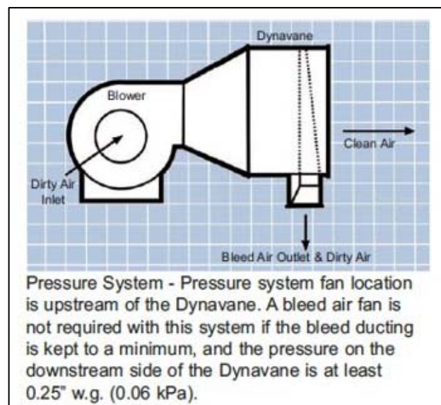
Figure 6: Dynavane Pressure System
