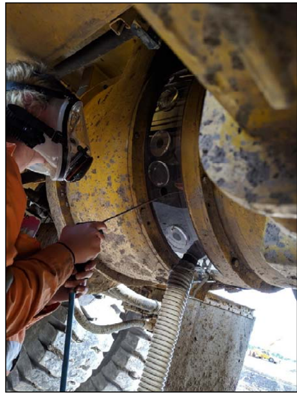
Photo 34: Separation screens between dust generating activity and CMW (alternator)
